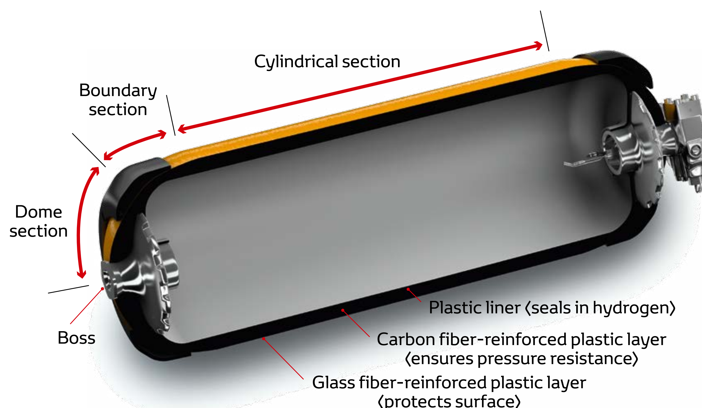
High-pressure hydrogen tank
